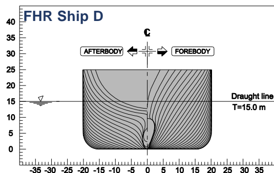
Fig. 1. Body plans and rendered views of the container ships.
