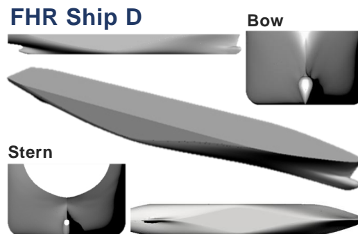
Fig. 1. Body plans and rendered views of the container ships.
