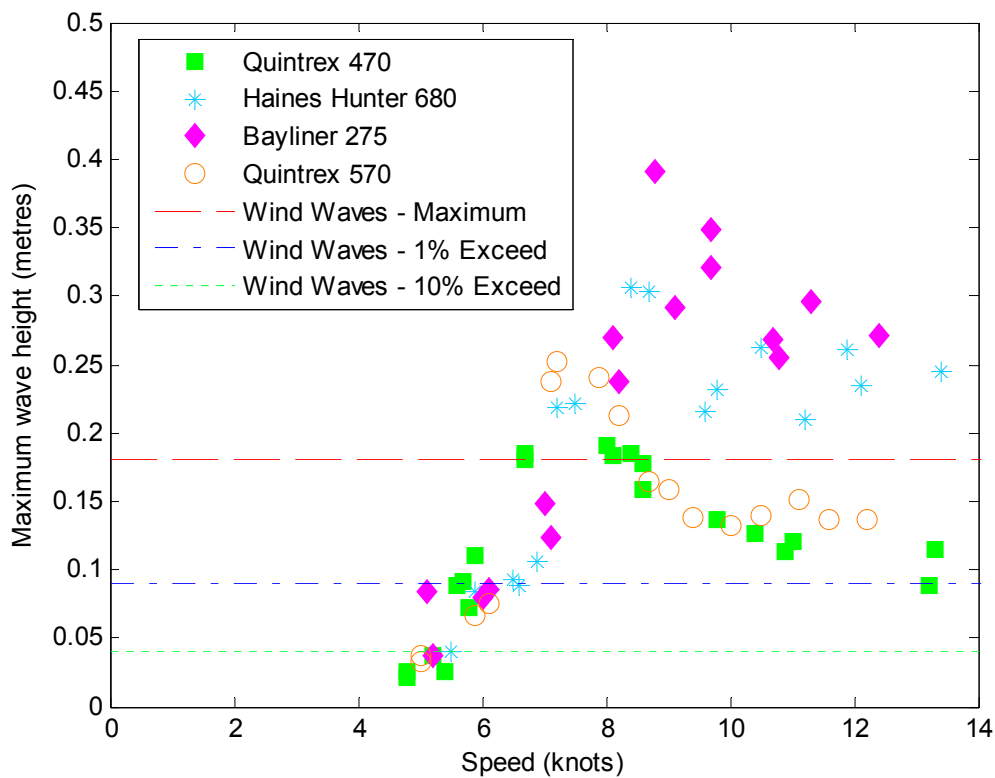
Figure 16: Measured maximum wave height for all close-approach trials at Ashfield Parade
