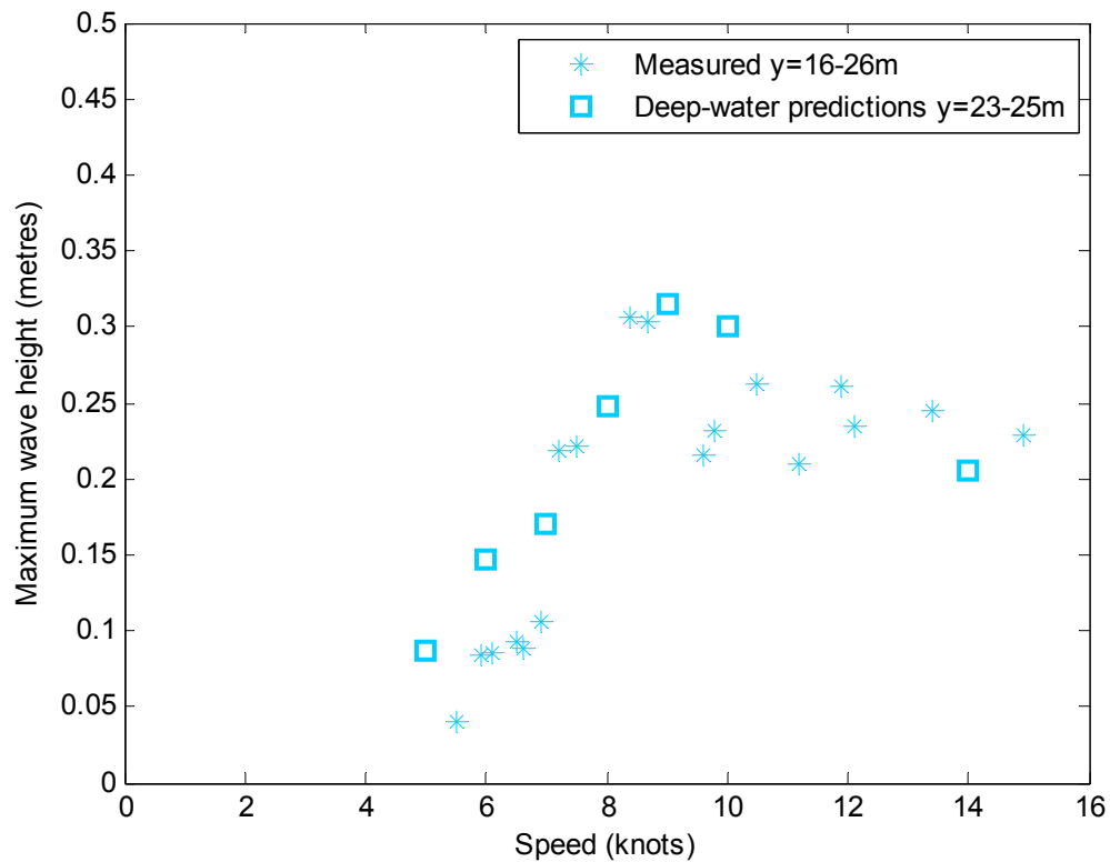
Figure 28: Comparison between measured wave heights and deep-water predictions for close-approach trials of Haines Hunter 680 at Ashfield Parade
