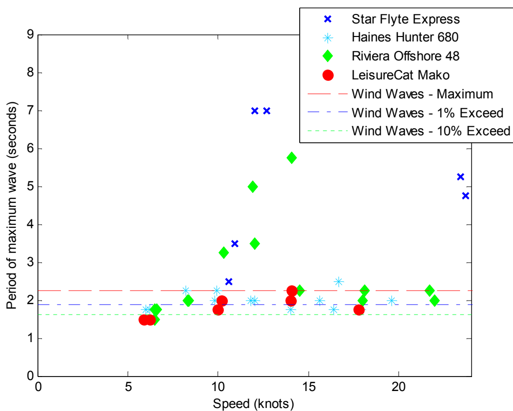
Figure 46: Measured period of maximum wave for all distant-approach trials at Quarry Point
