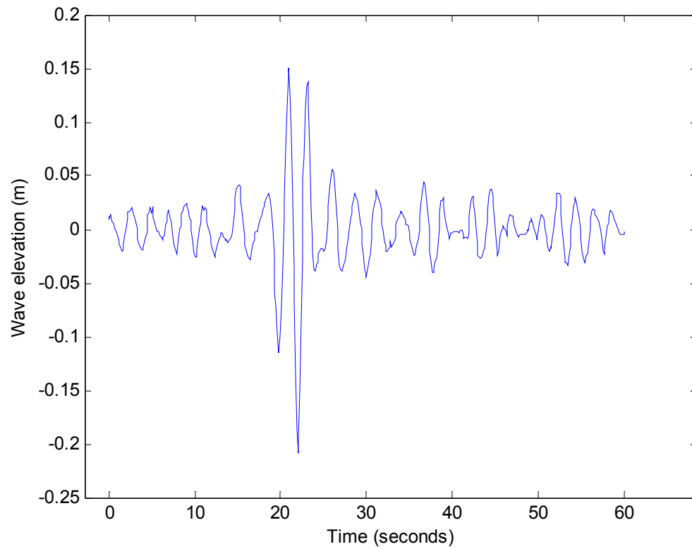
Figure 34: Wave elevation for Haines Hunter Patriot 680 example case (largest wave height): 7.6 knots at 09:57
