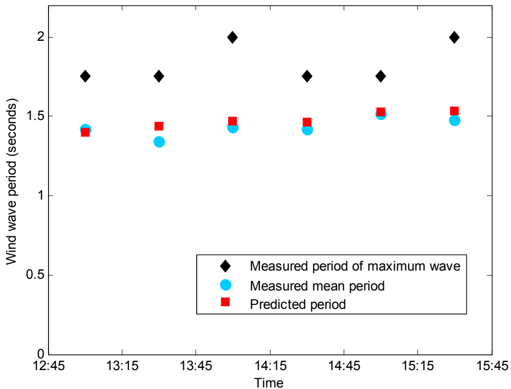
Figure 102: Measured wind wave periods, together with wave period predictions, over 30-minute intervals during wind wave trials at Quarry Point on 12 th Feb 2010
