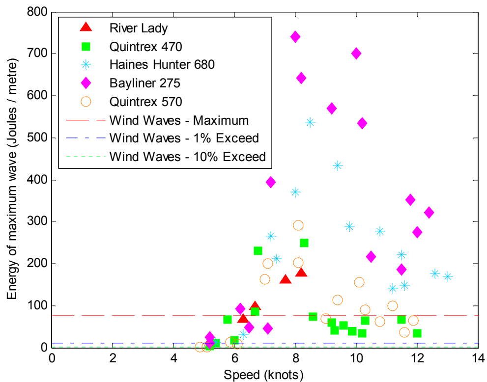
Figure 26: Measured energy of maximum wave for all distant-approach trials at Ashfield Parade
