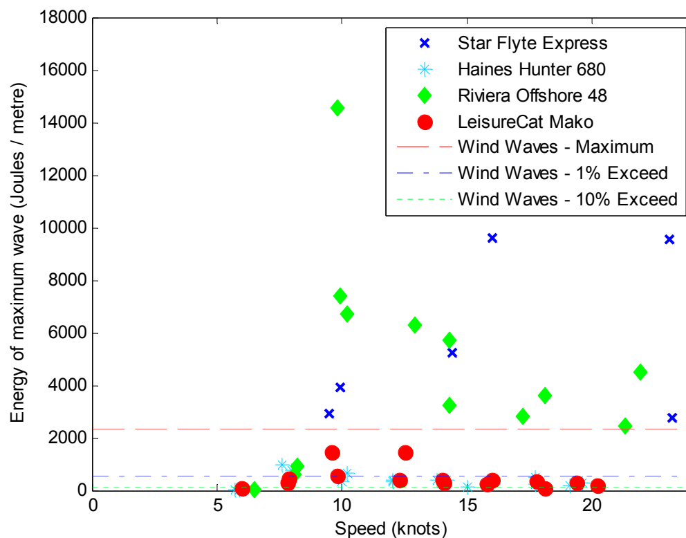
Figure 51: Measured energy of maximum wave for all close-approach trials at Quarry Point
