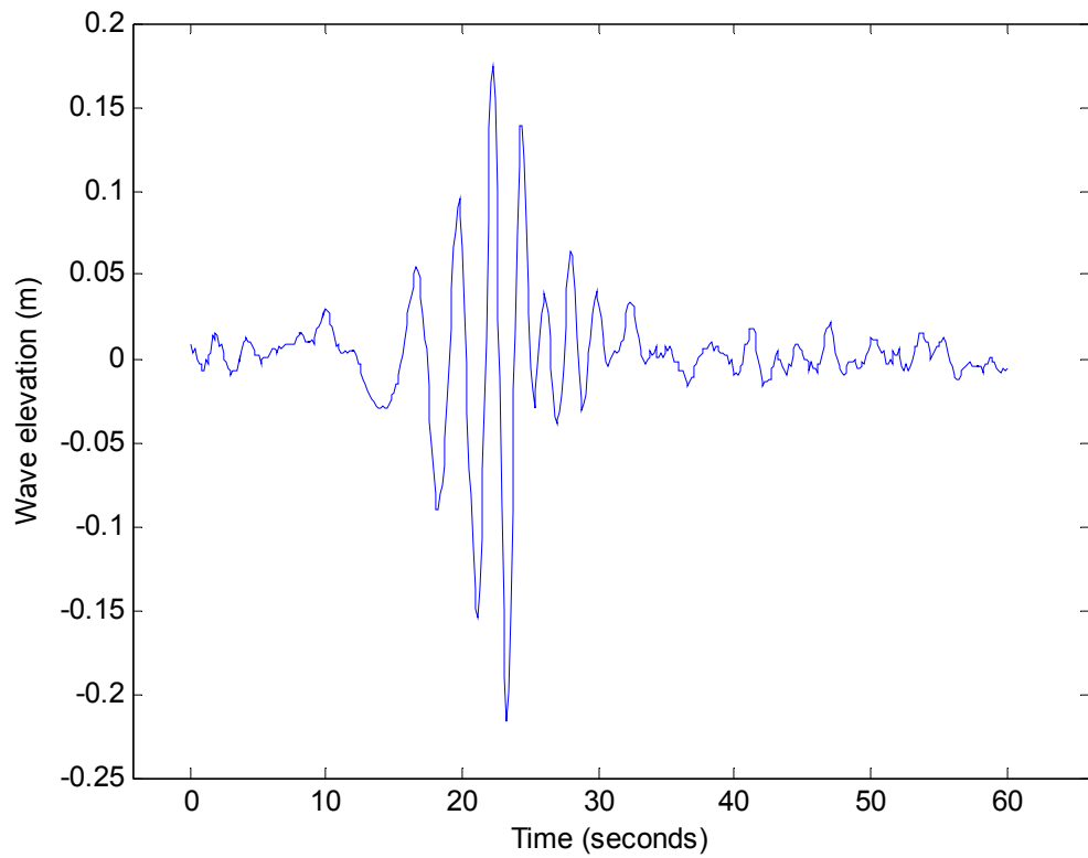
Figure 8: Measured wave elevation for Bayliner 275 example case (largest wave height): 8.8 knots at 07:01
