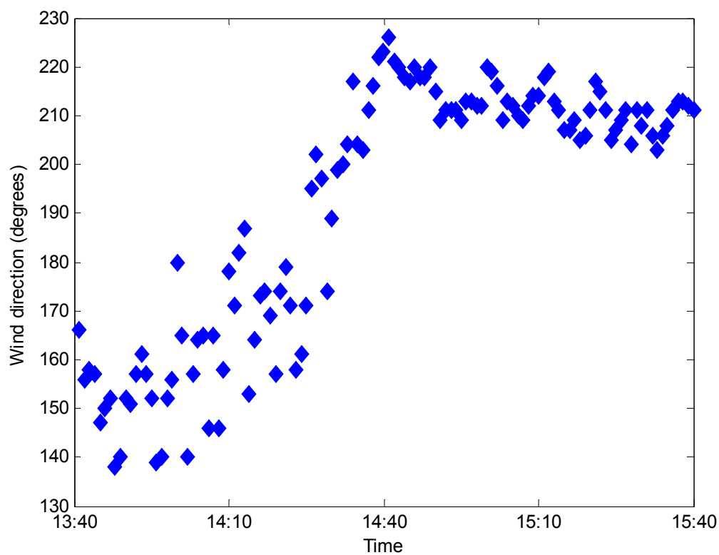
Figure 86: Measured wind direction at Melville Water during wind wave trials at Ashfield Parade on 3 rd Feb 2010
