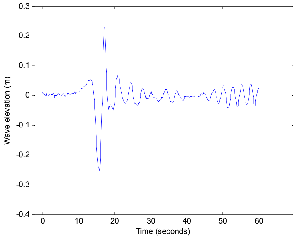
Figure 64: Wave elevation for Noel Robins example case (largest wave height): 7.9 knots at 13:39
