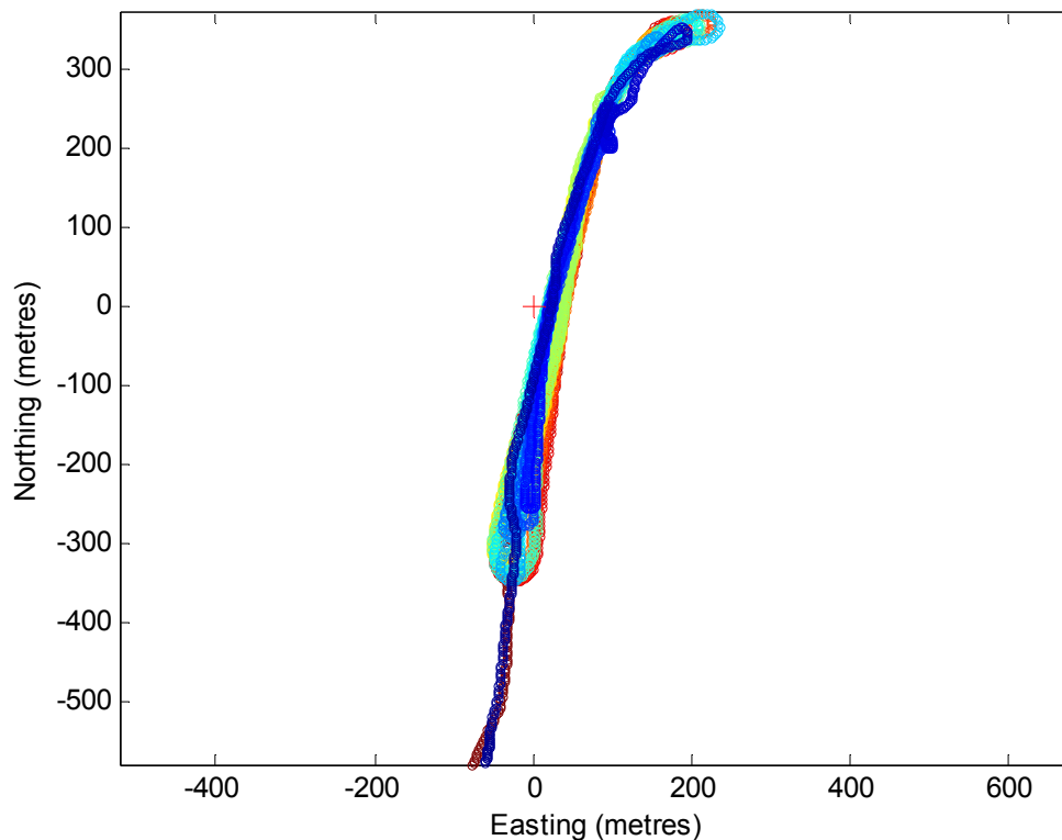
Figure 7: Example GPS trace from Ashfield Parade, for Haines Hunter 680. GPS positions shown relative to waver recorder (red cross). Colours show times, from blue (start) to red (end).
