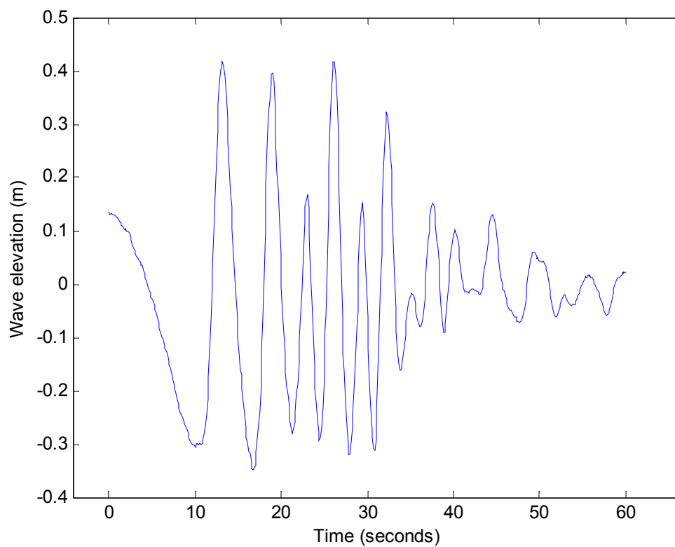
Figure 36: Wave elevation for Star Flyte Express example case (largest wave height): 12.0 knots at 06:48
