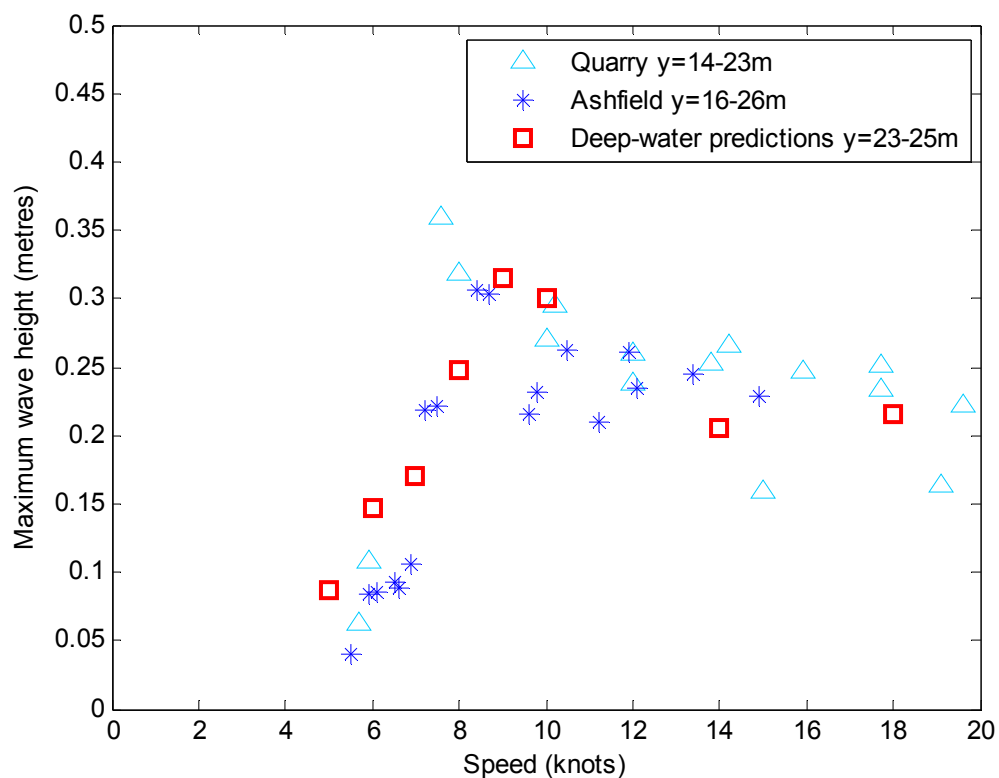
Figure 55: Comparison between measured wave heights and deep-water predictions for close-approach trials of Haines Hunter 680 at Quarry Point. Ashfield Parade results for Haines Hunter 680 also shown.
