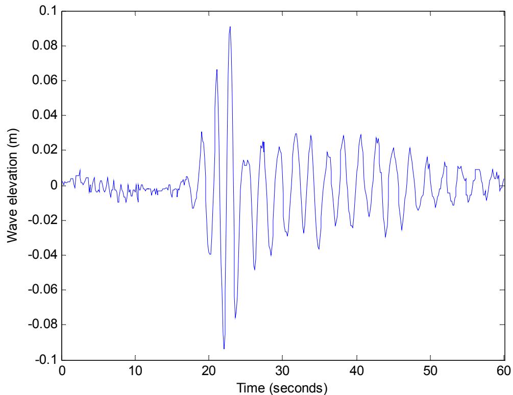
Figure 11: Measured wave elevation for Quintrex Freedom Sport 470 example case (largest wave height): 6.7 knots at 07:06
