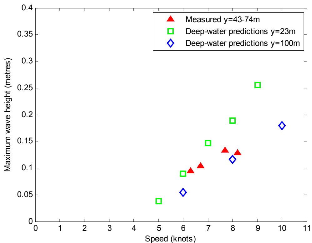
Figure 30: Comparison between measured wave heights and deep-water predictions for River Lady at Ashfield Parade
