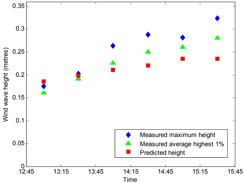
Figure 101: Measured wind wave heights, together with wave height predictions, over 30-minute intervals during wind wave trials at Quarry Point on 12 th Feb 2010
