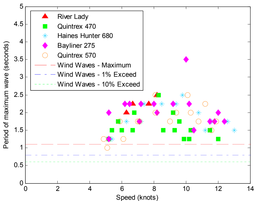
Figure 19: Measured period of maximum wave for all distant-approach trials at Ashfield Parade
