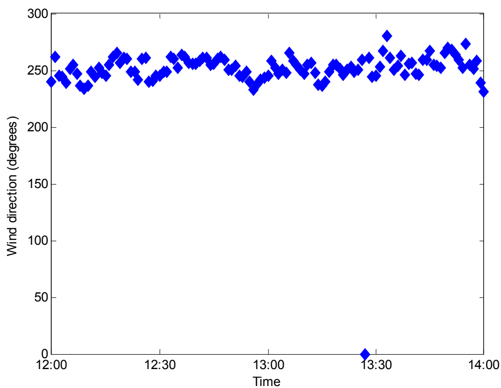
Figure 93: Measured wind direction at Melville Water during wind wave trials at Quarry Point on 11 th Feb 2010
