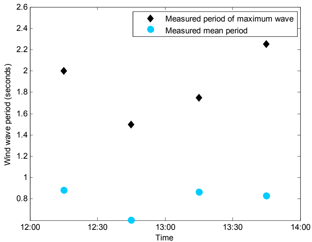
Figure 96: Measured wind wave periods over 30-minute intervals during wind wave trials at Quarry Point on 11 th Feb 2010
