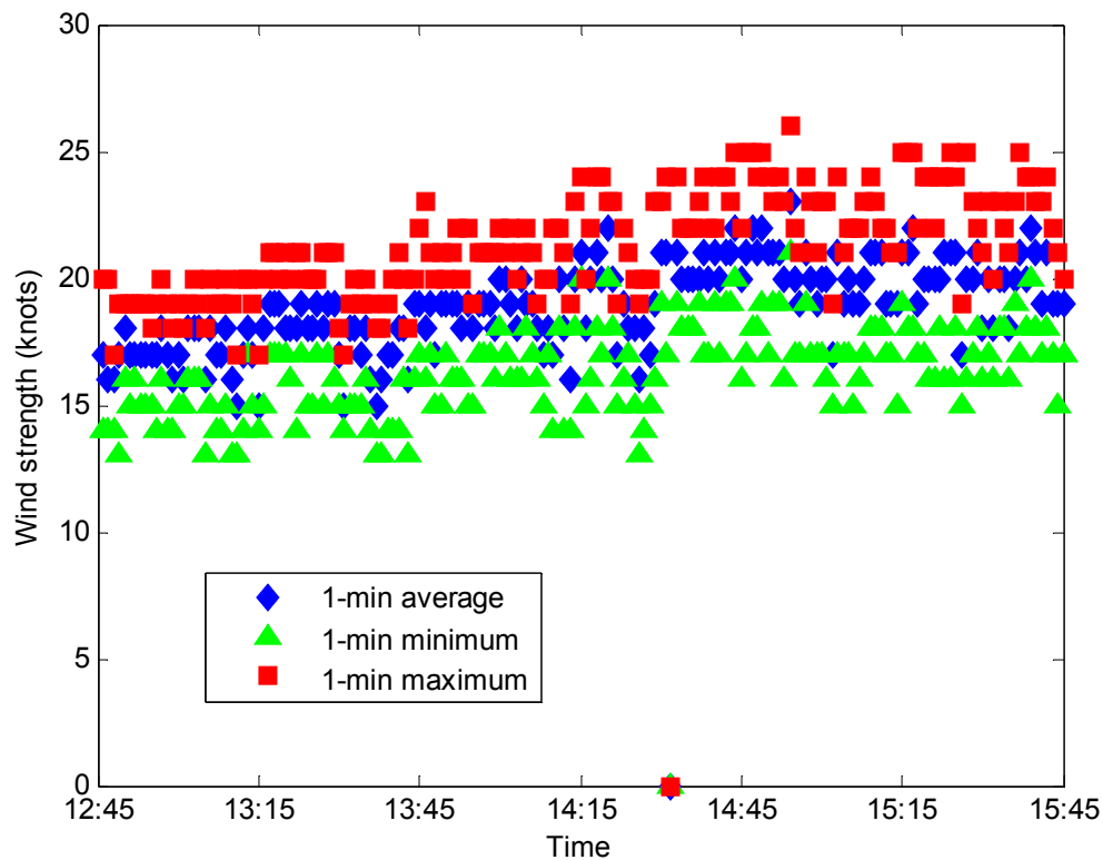
Figure 97: Measured wind strength at Melville Water during wind wave trials at Quarry Point on 12 th Feb 2010
