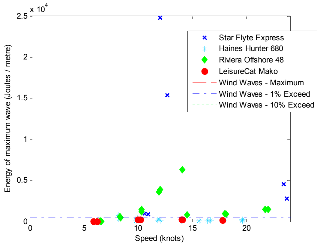
Figure 53: Measured energy of maximum wave for all distant-approach trials at Quarry Point
