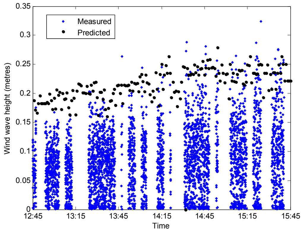
Figure 100: Measured individual wind wave heights, together with wave height predictions, during wind wave trials at Quarry Point on 12 th Feb 2010
