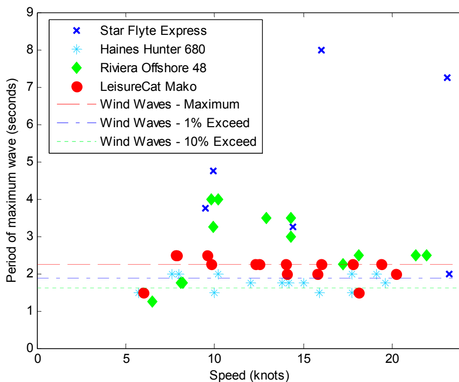
Figure 45: Measured period of maximum wave for all close-approach trials at Quarry Point
