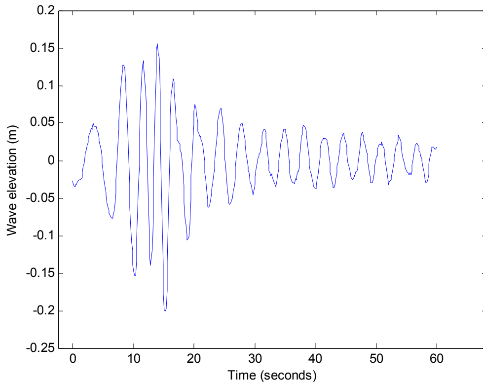
Figure 41: Wave elevation for LeisureCat Mako 9000 example case (largest wave height): 9.6 knots at 09:29
