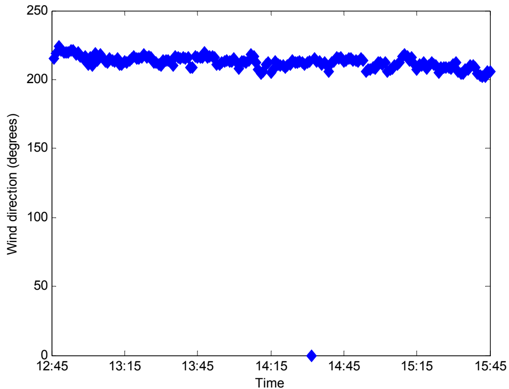
Figure 98: Measured wind direction at Melville Water during wind wave trials at Quarry Point on 12 th Feb 2010
