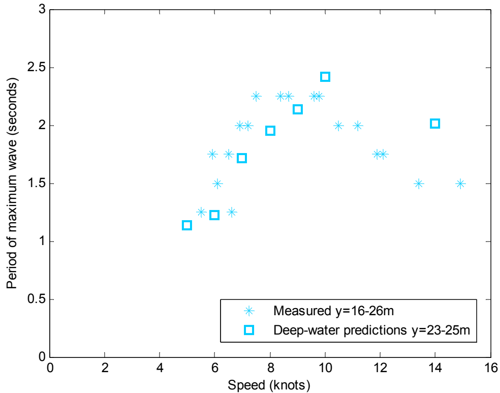
Figure 29: Comparison between measured wave periods and deep-water predictions for close-approach trials of Haines Hunter 680 at Ashfield Parade
