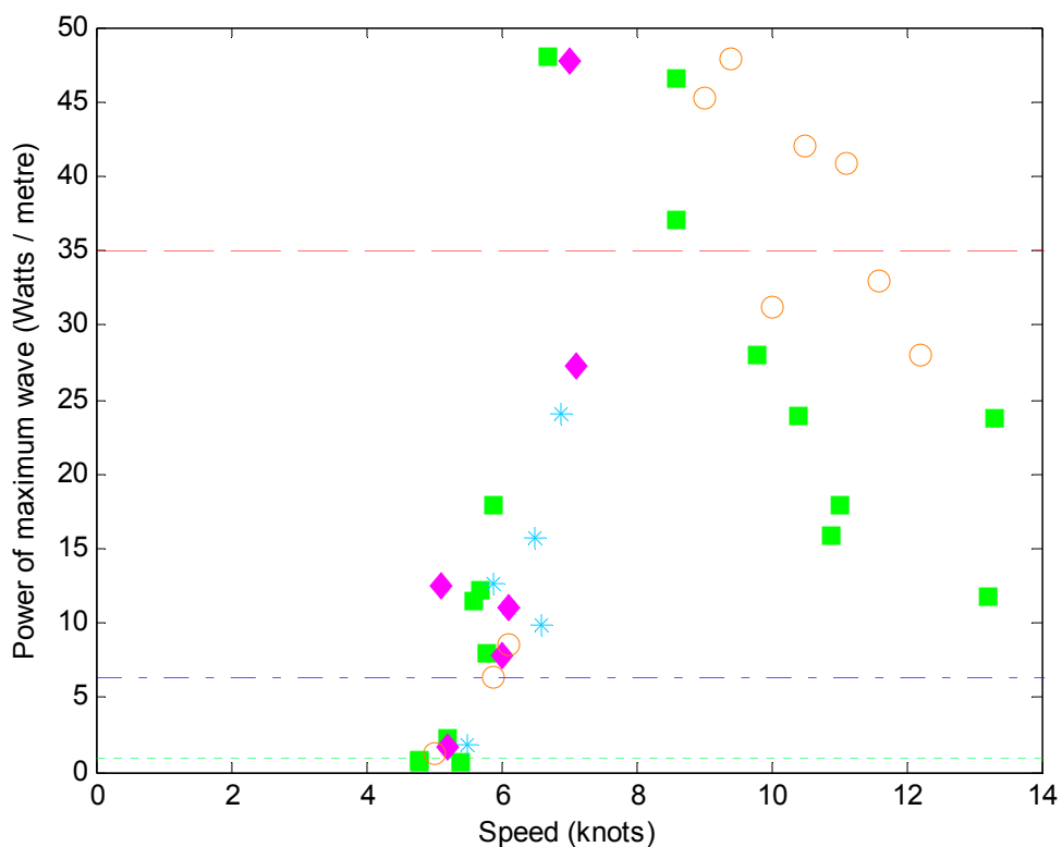
Figure 21: Measured power of maximum wave for all close-approach trials at Ashfield Parade: zoomed in
