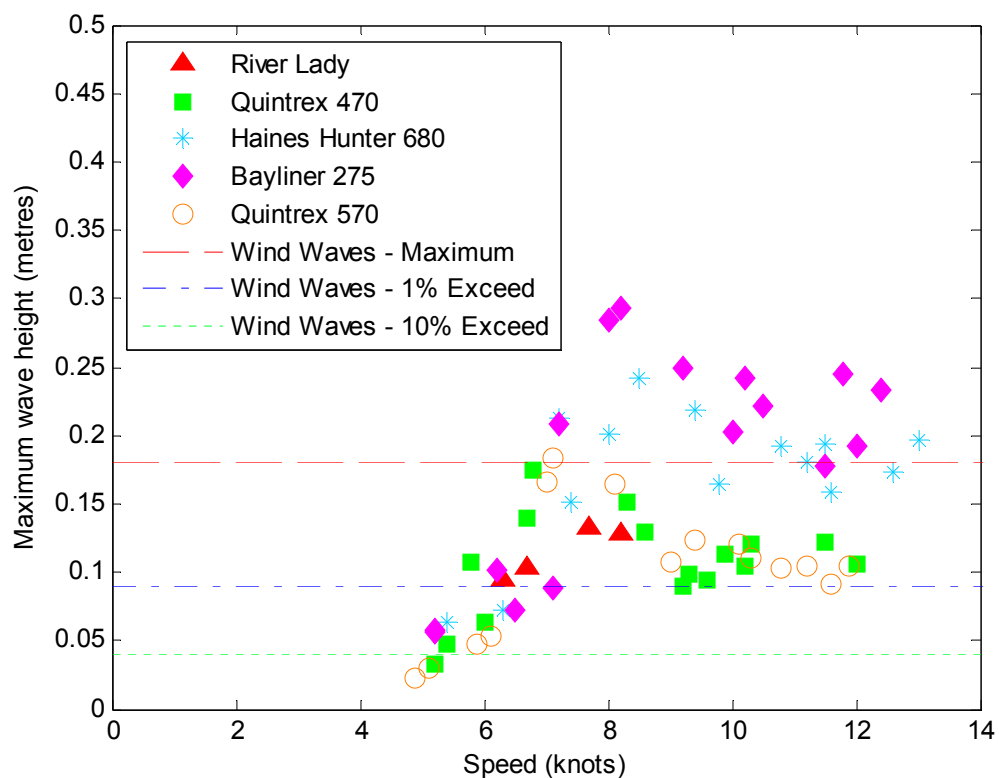
Figure 17: Measured maximum wave height for all distant-approach trials at Ashfield Parade
