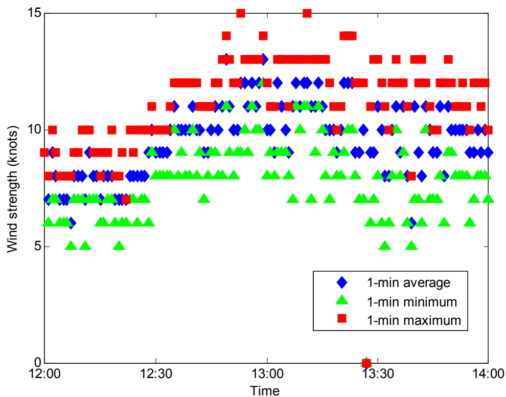
Figure 92: Measured wind strength at Melville Water during wind wave trials at Quarry Point on 11 th Feb 2010
