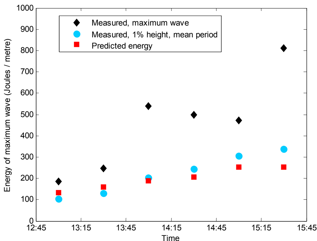
Figure 104: Measured energy of maximum wind waves, together with predictions, over 30-minute intervals during wind wave trials at Quarry Point on 12 th Feb 2010
