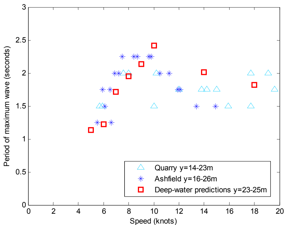
Figure 56: Comparison between measured wave periods and deep-water predictions for close-approach trials of Haines Hunter 680 at Quarry Point. Ashfield Parade results for Haines Hunter 680 also shown.
