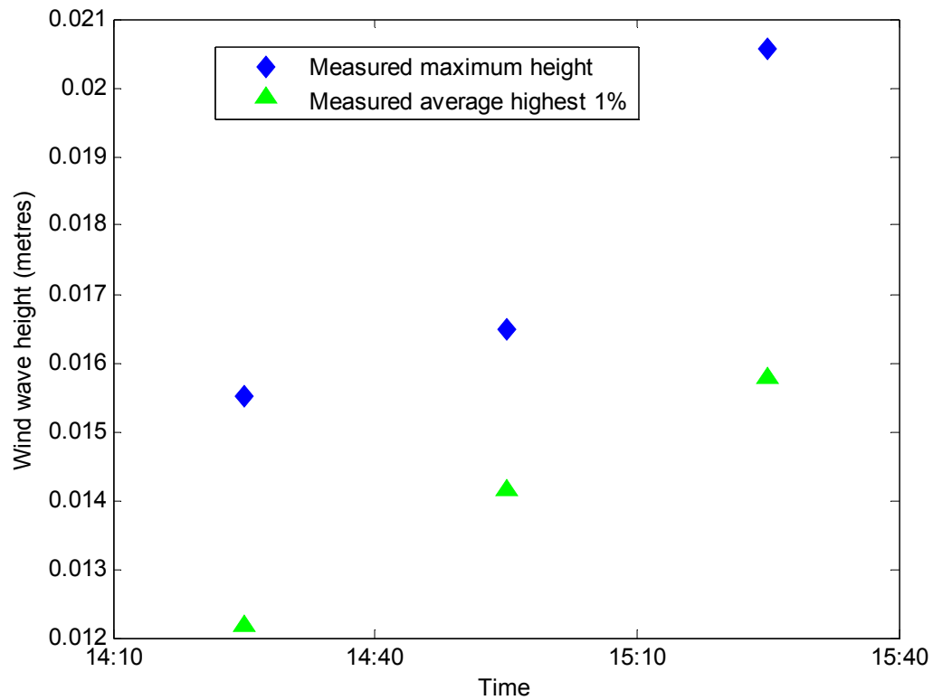
Figure 83: Measured wind wave heights over 30-minute intervals during wind wave trials at Ashfield Parade on 2 nd Feb 2010
