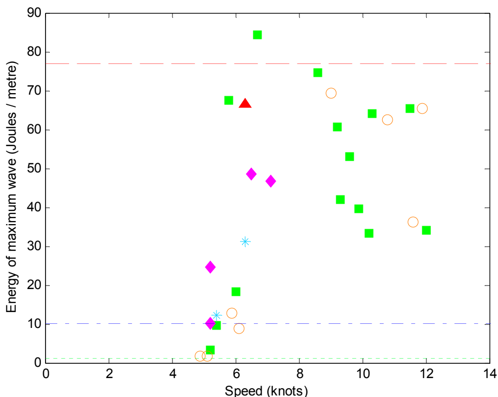
Figure 27: Measured energy of maximum wave for all distant-approach trials at Ashfield Parade: zoomed in
