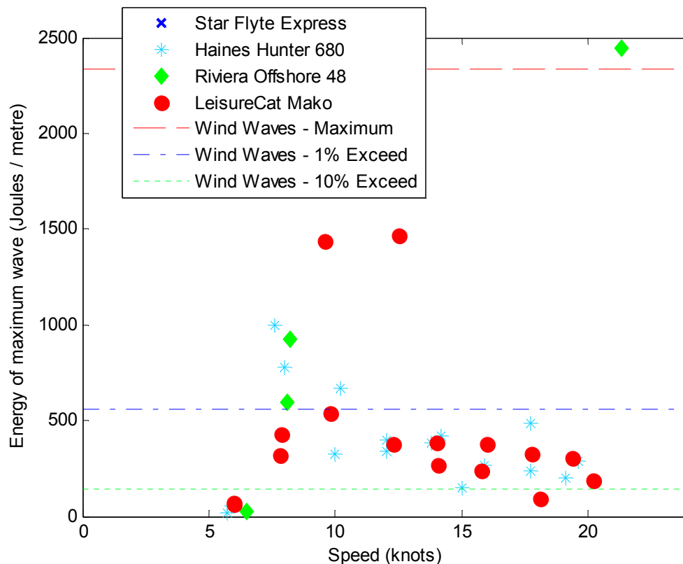
Figure 52: Measured energy of maximum wave for all close-approach trials at Quarry Point: zoomed in
