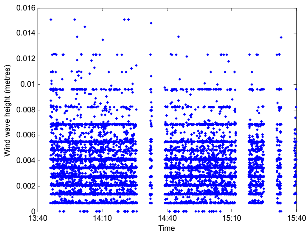
Figure 87: Measured individual wind wave heights during wind wave trials at Ashfield Parade on 3 rd Feb 2010
