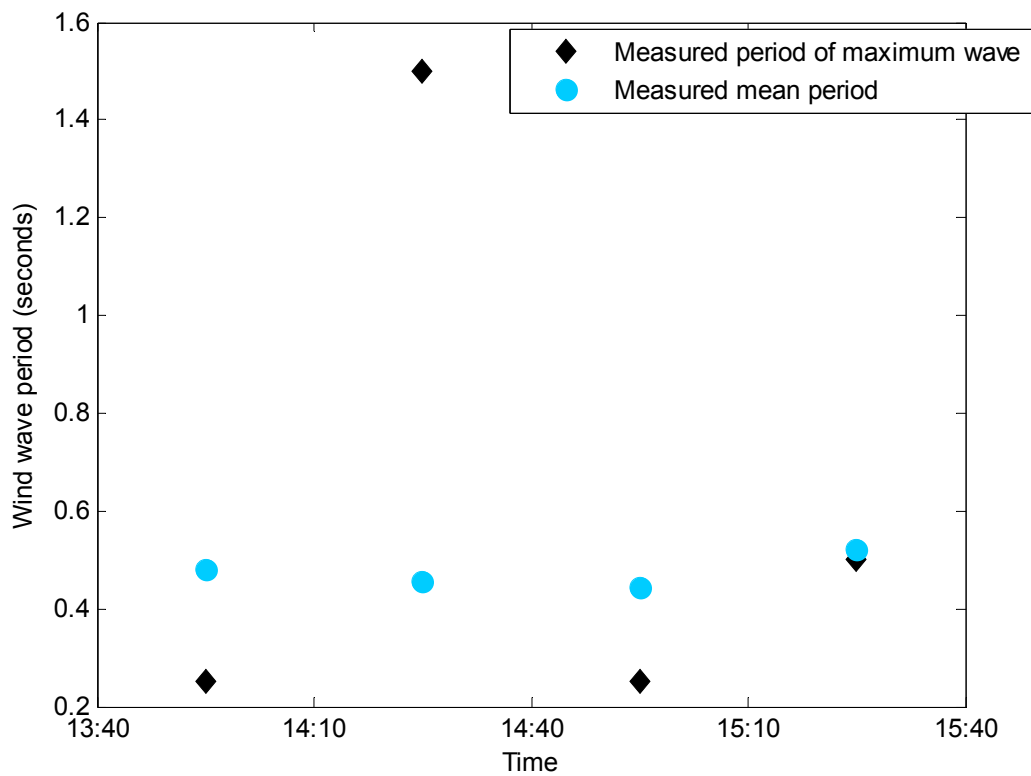
Figure 89: Measured wind wave periods over 30-minute intervals during wind wave trials at Ashfield Parade on 3 rd Feb 2010
