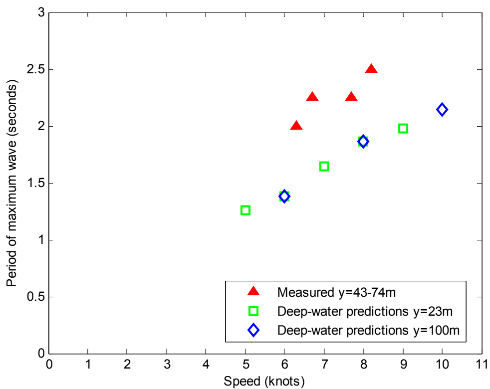
Figure 31: Comparison between measured wave periods and deep-water predictions for River Lady at Ashfield Parade
