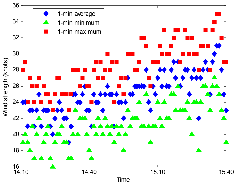
Figure 80: Measured wind strength at Melville Water during wind wave trials at Ashfield Parade on 2 nd Feb 2010
