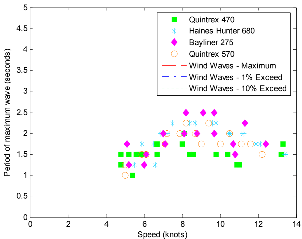
Figure 18: Measured period of maximum wave for all close-approach trials at Ashfield Parade
