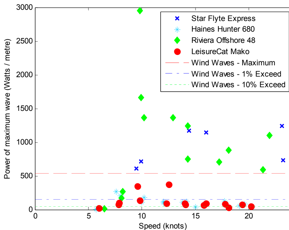
Figure 47: Measured power of maximum wave for all close-approach trials at Quarry Point
