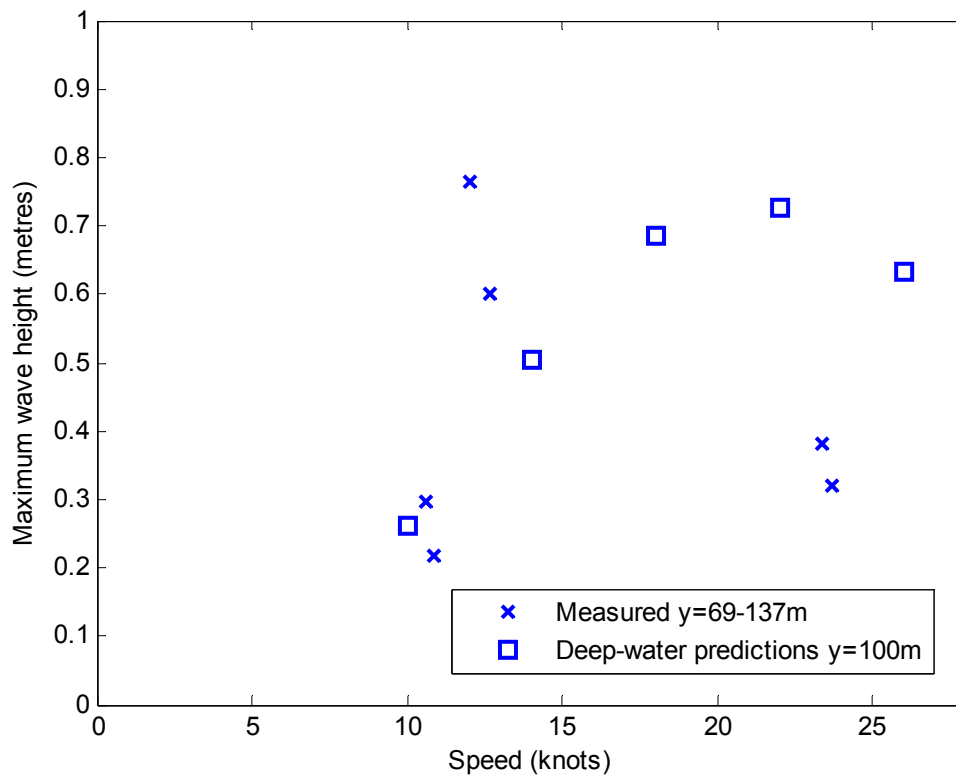
Figure 61: Comparison between measured wave heights and deep-water predictions for distant-approach trials of Star Flyte Express at Quarry Point
