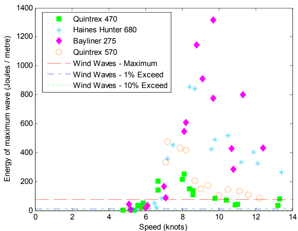
Figure 24: Measured energy of maximum wave for all close-approach trials at Ashfield Parade
