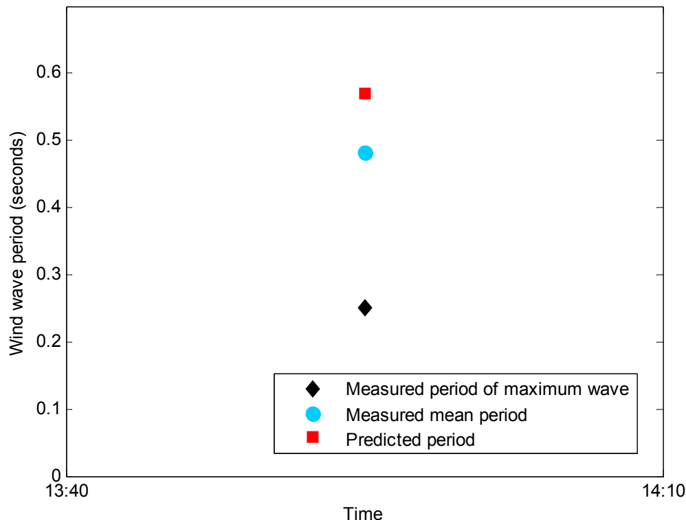
Figure 91: Measured and predicted wind wave periods over 30-minute interval during wind wave trials at Ashfield Parade on 3 rd Feb 2010
