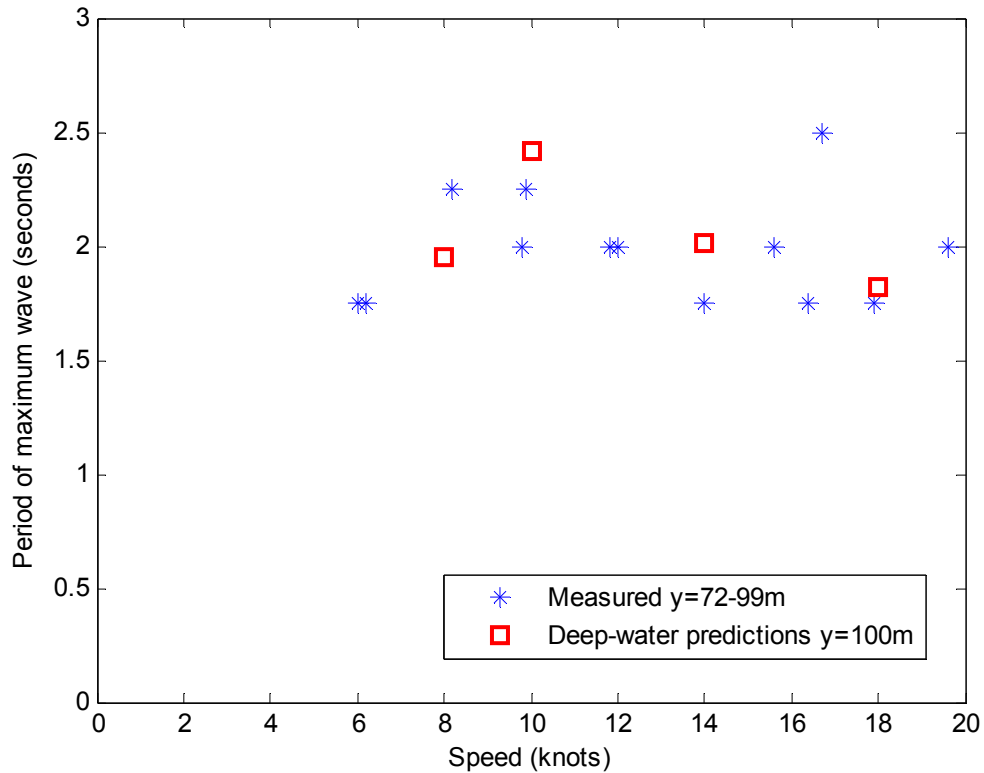
Figure 58: Comparison between measured wave periods and deep-water predictions for distant-approach trials of Haines Hunter 680 at Quarry Point
