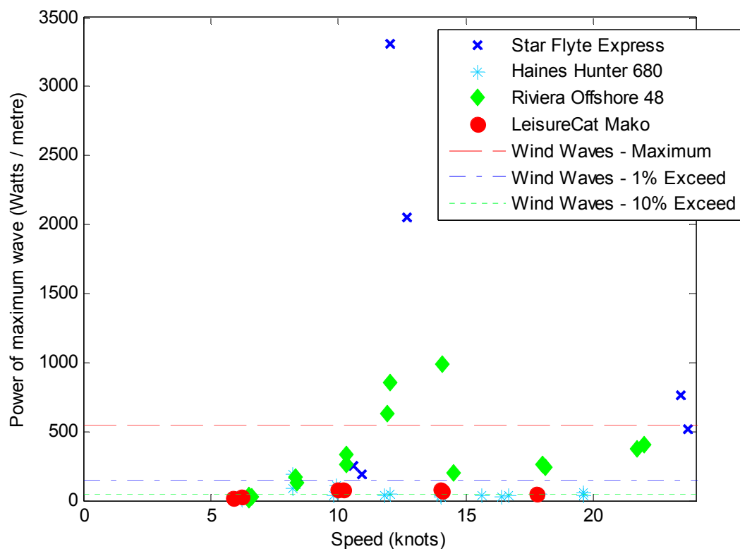
Figure 49: Measured power of maximum wave for all distant-approach trials at Quarry Point
