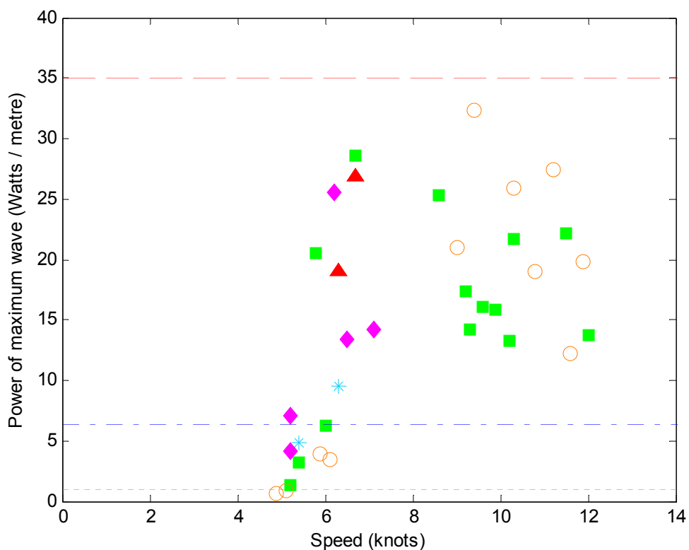
Figure 23: Measured power of maximum wave for all distant-approach trials at Ashfield Parade: zoomed in
