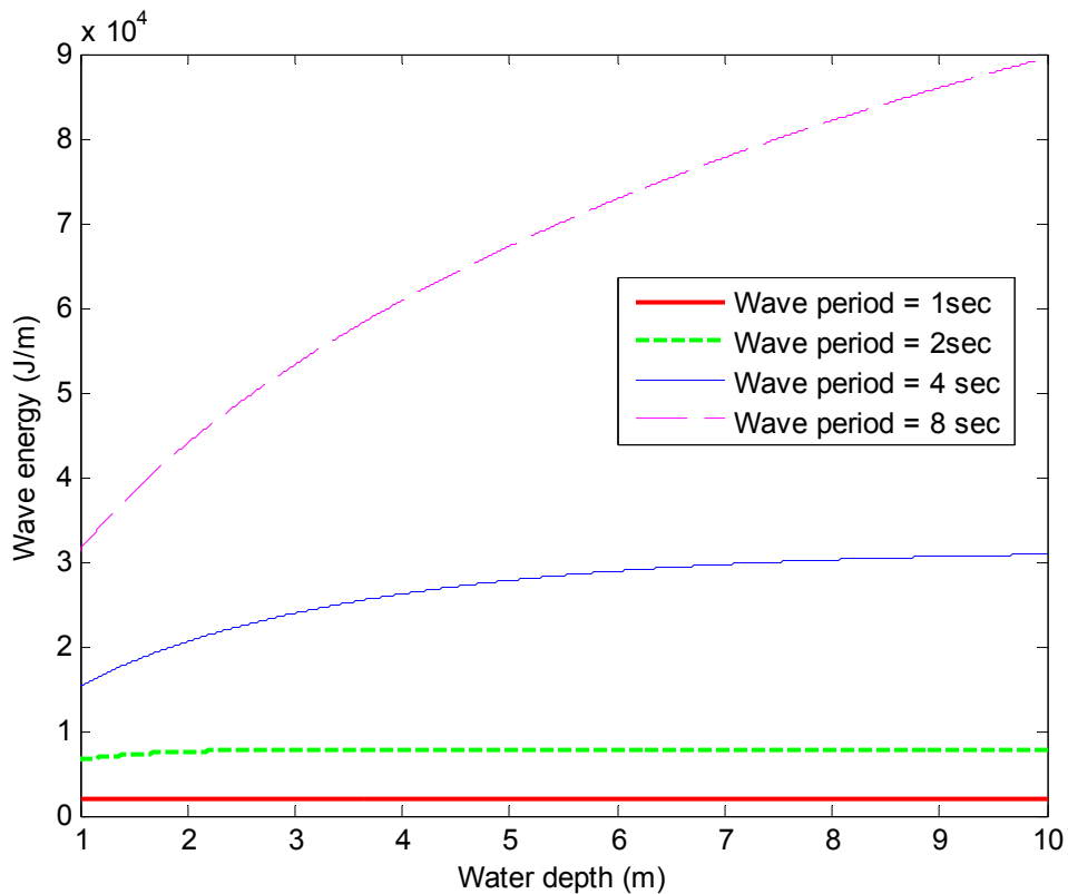
Figure 106: Effect of water depth on energy per wavelength, for different wave periods. Based on linear wave height = 1.0m.
