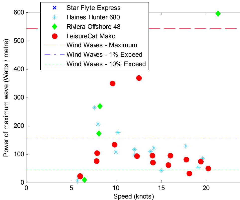
Figure 48: Measured power of maximum wave for all close-approach trials at Quarry Point: zoomed in
