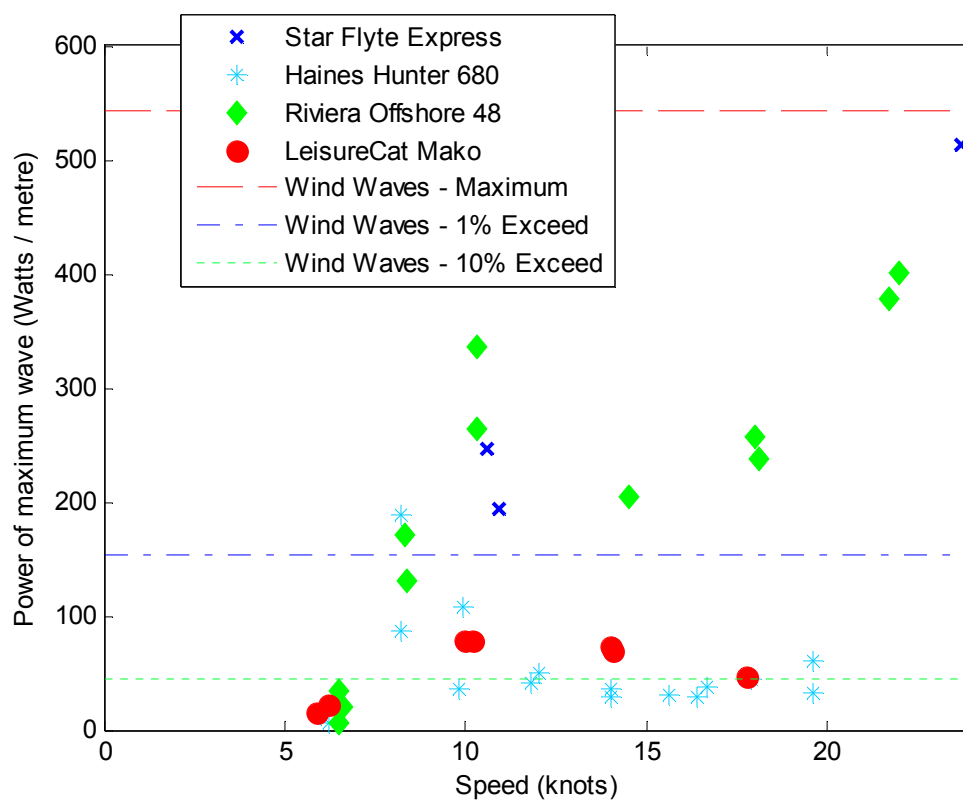
Figure 50: Measured power of maximum wave for all distant-approach trials at Quarry Point: zoomed in
