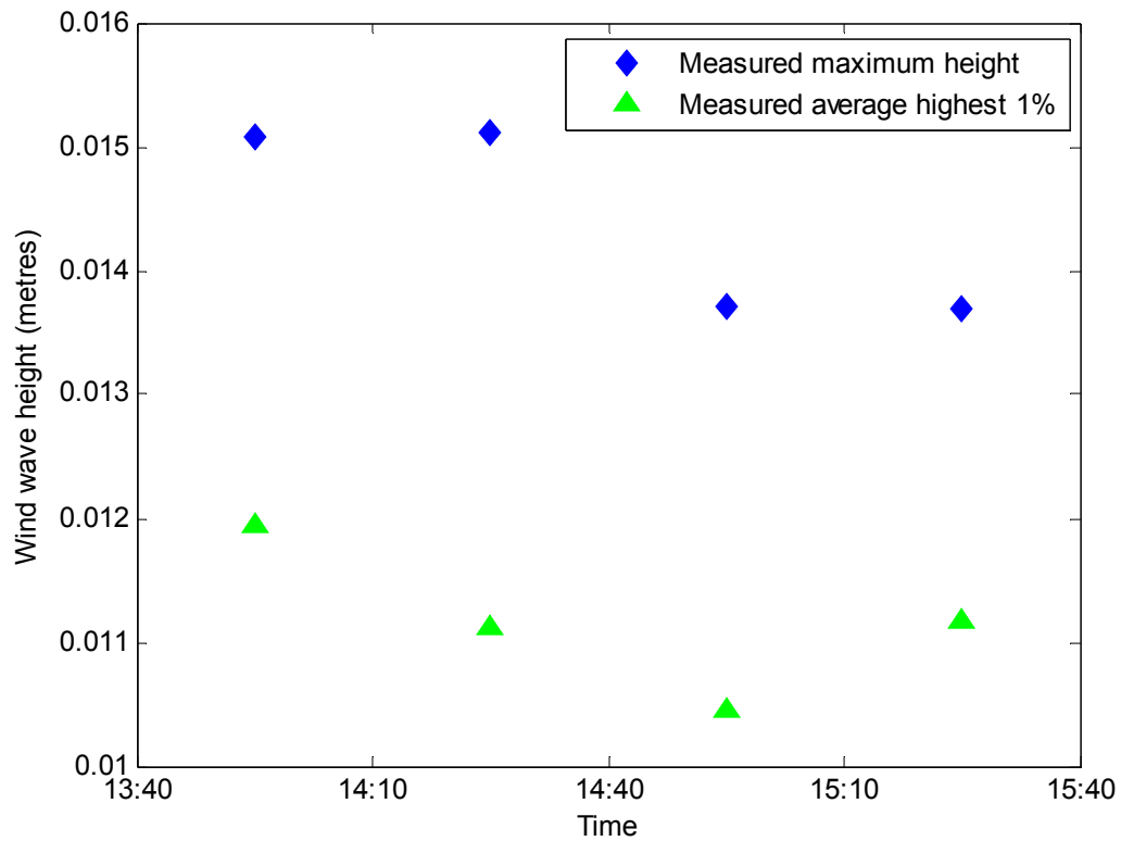
Figure 88: Measured wind wave heights over 30-minute intervals during wind wave trials at Ashfield Parade on 3 rd Feb 2010
