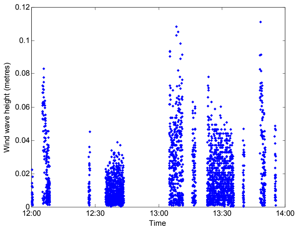
Figure 94: Measured individual wind wave heights during wind wave trials at Quarry Point on 11 th Feb 2010
