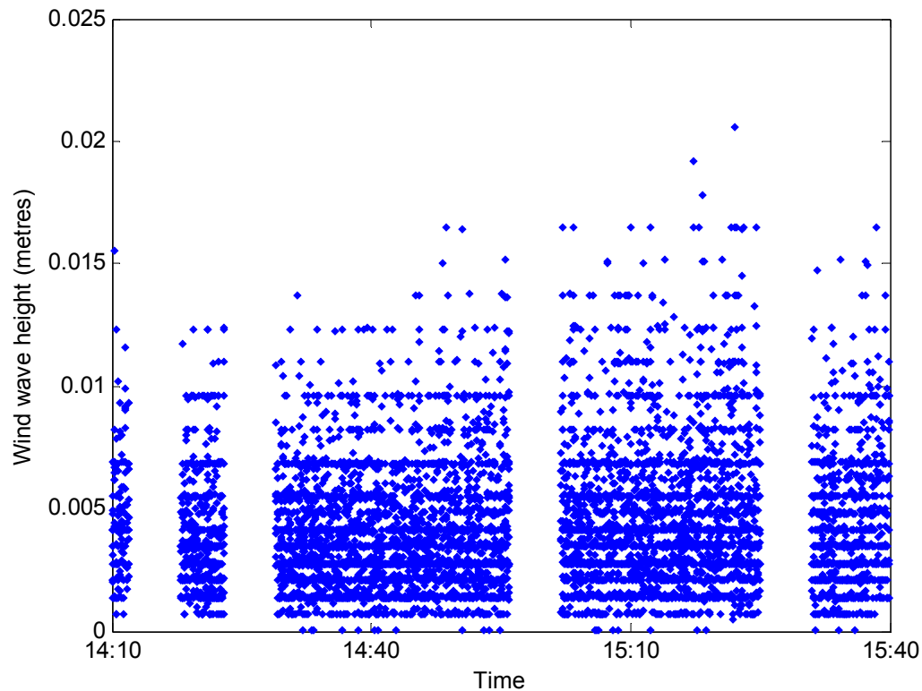
Figure 82: Measured individual wind wave heights during wind wave trials at Ashfield Parade on 2 nd Feb 2010
