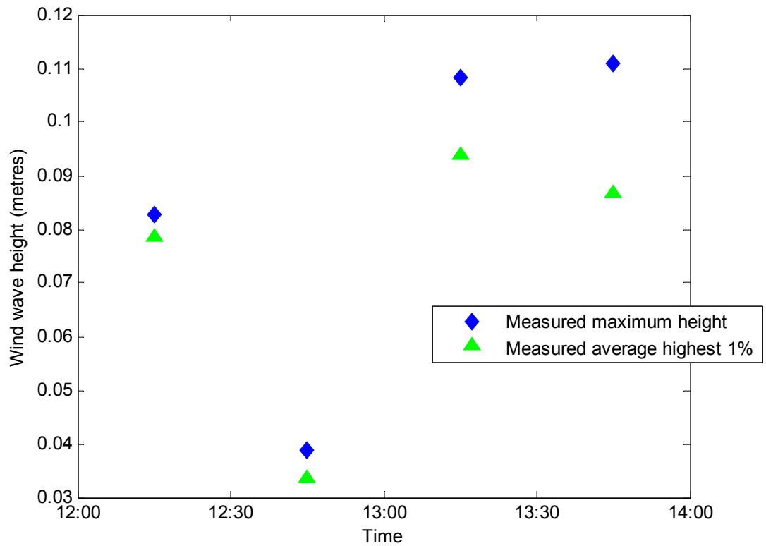
Figure 95: Measured wind wave heights over 30-minute intervals during wind wave trials at Quarry Point on 11 th Feb 2010
