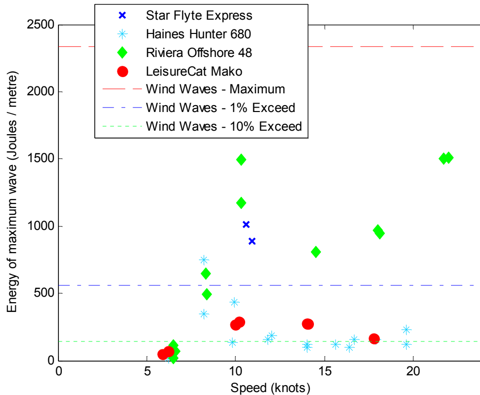
Figure 54: Measured energy of maximum wave for all distant-approach trials at Quarry Point: zoomed in
