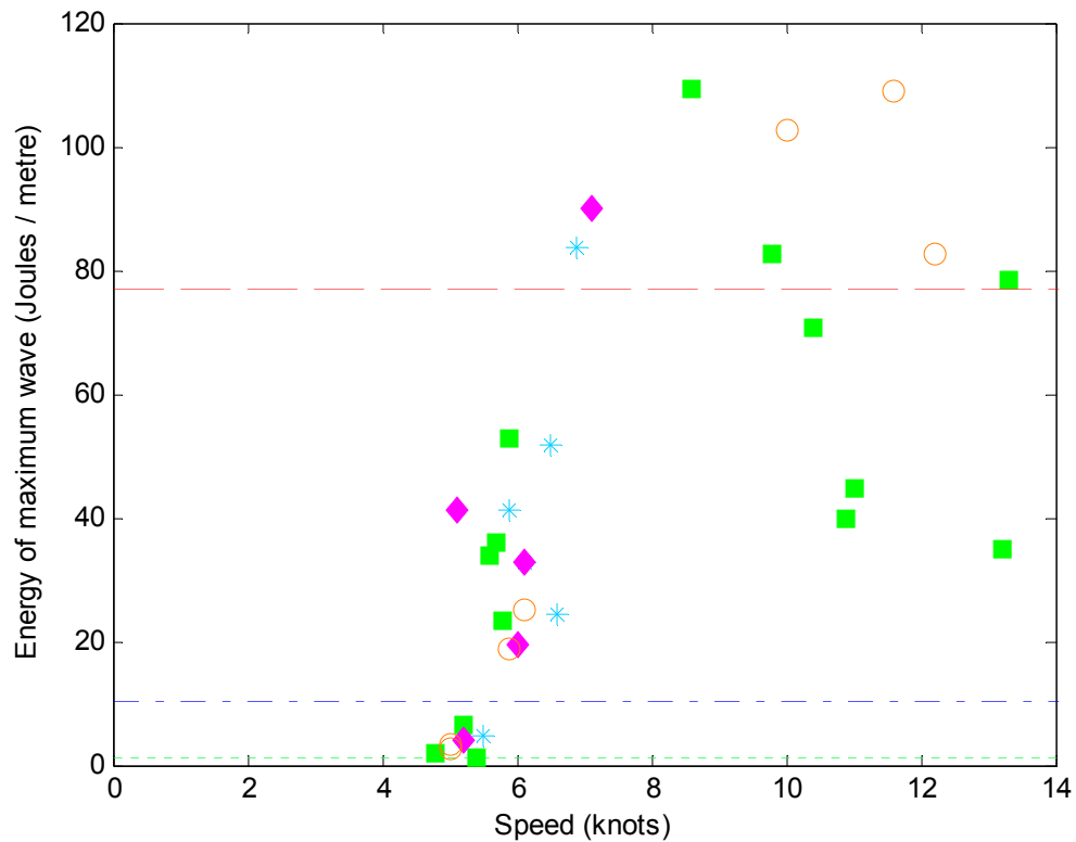
Figure 25: Measured energy of maximum wave for all close-approach trials at Ashfield Parade: zoomed in
