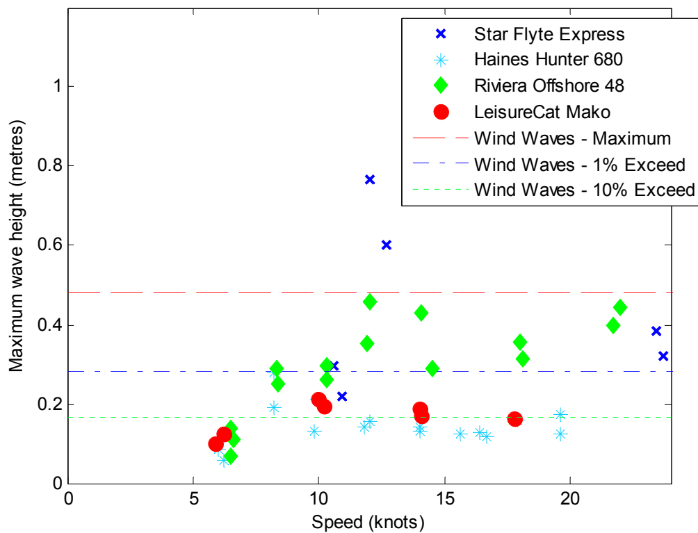
Figure 44: Measured maximum wave height for all distant-approach trials at Quarry Point
