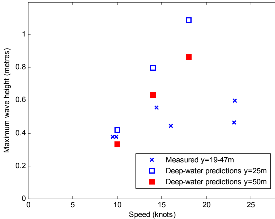
Figure 59: Comparison between measured wave heights and deep-water predictions for close-approach trials of Star Flyte Express at Quarry Point
