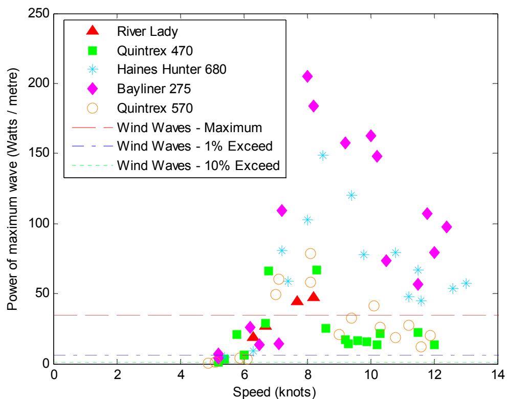
Figure 22: Measured power of maximum wave for all distant-approach trials at Ashfield Parade
