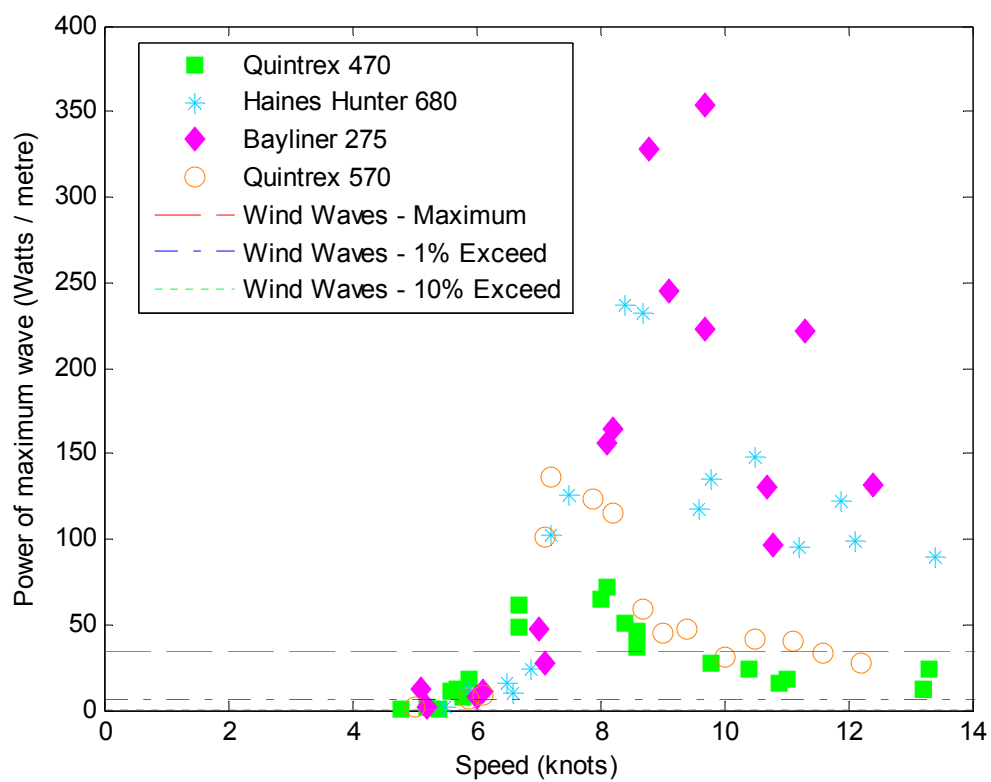
Figure 20: Measured power of maximum wave for all close-approach trials at Ashfield Parade
