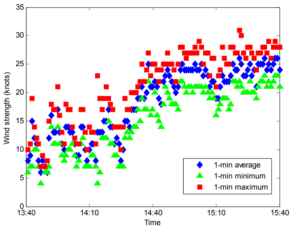
Figure 85: Measured wind strength at Melville Water during wind wave trials at Ashfield Parade on 3 rd Feb 2010
