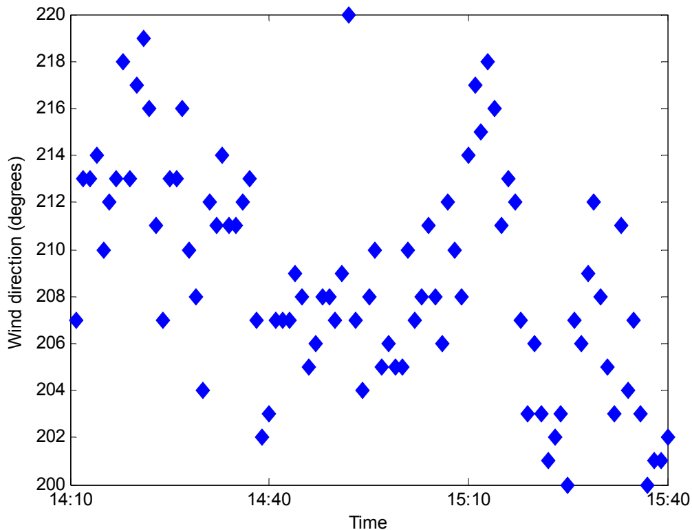
Figure 81: Measured wind direction at Melville Water during wind wave trials at Ashfield Parade on 2 nd Feb 2010
