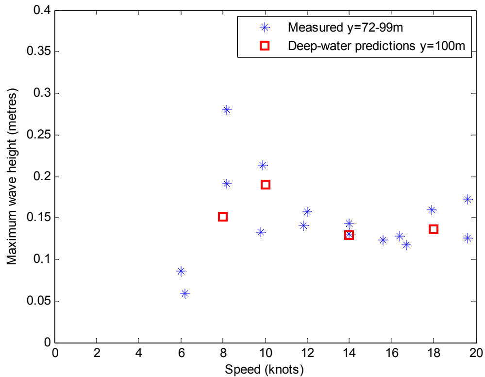
Figure 57: Comparison between measured wave heights and deep-water predictions for distant-approach trials of Haines Hunter 680 at Quarry Point
