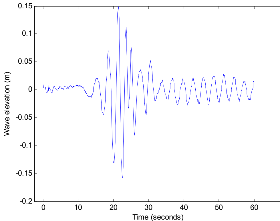
Figure 10: Measured wave elevation for Haines Hunter Patriot 680 example case (largest wave height): 8.4 knots at 09:18
