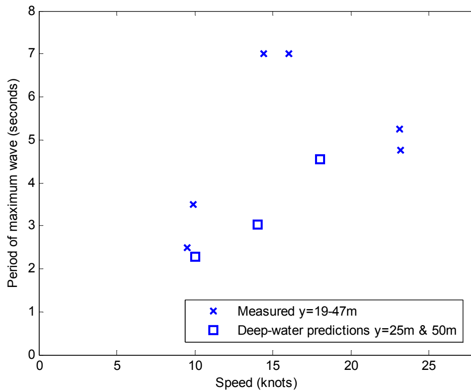
Figure 60: Comparison between measured wave periods and deep-water predictions for close-approach trials of Star Flyte Express at Quarry Point
