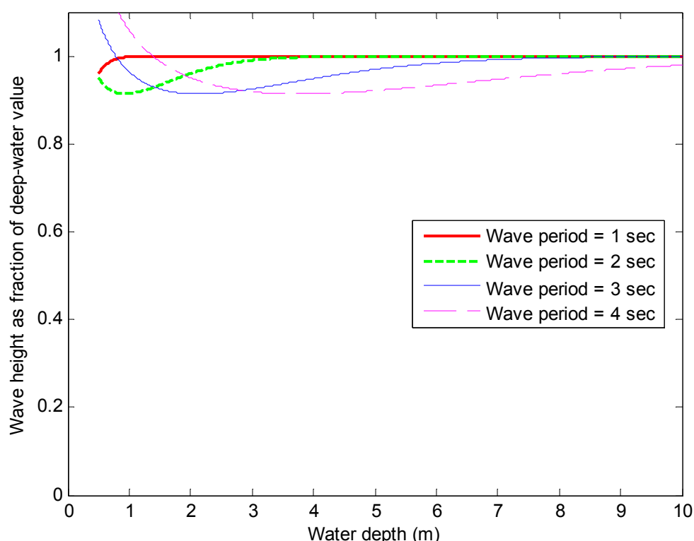
Figure 105: Changing wave height as a linear wave moves into shallower water
