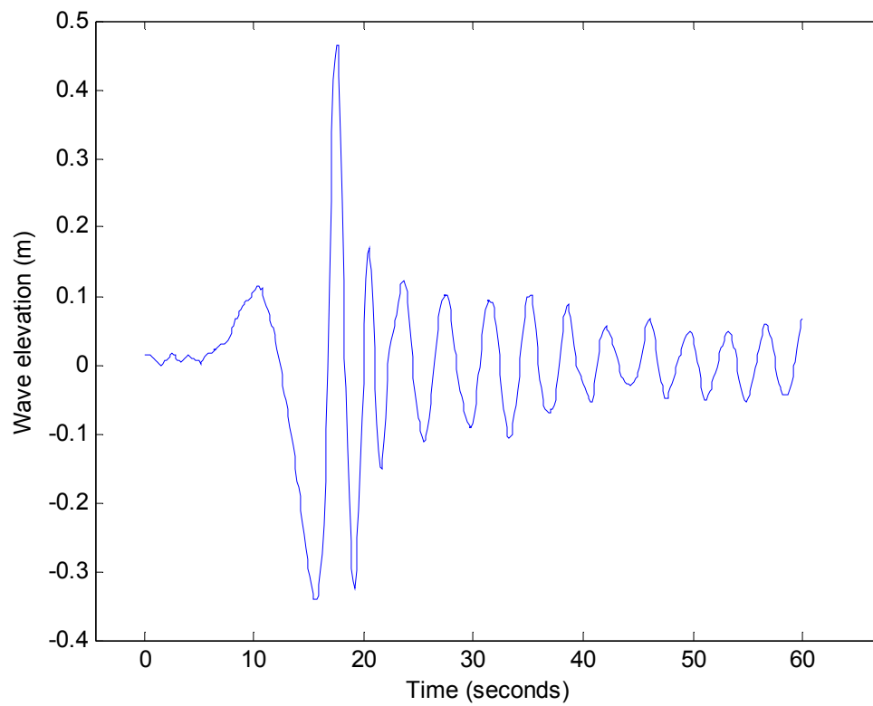
Figure 39: Wave elevation for Riviera Offshore Express 48 example case (largest wave height): 9.8 knots at 09:28
