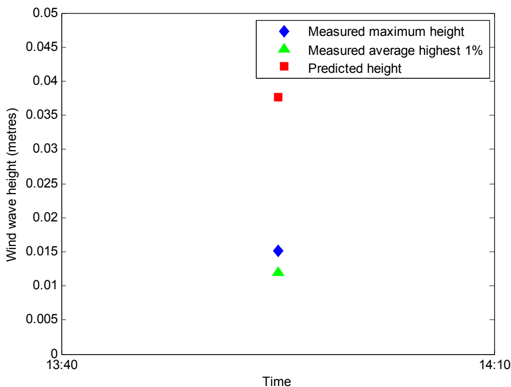
Figure 90: Measured and predicted wind wave heights over 30-minute interval during wind wave trials at Ashfield Parade on 3 rd Feb 2010
