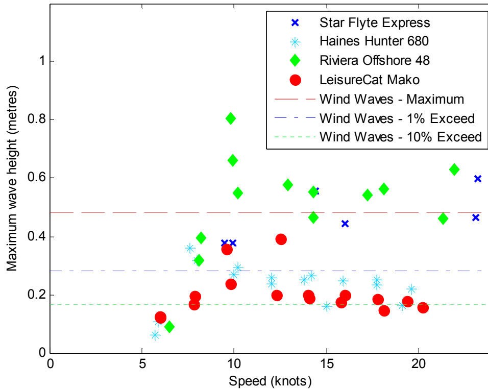
Figure 43: Measured maximum wave height for all close-approach trials at Quarry Point
