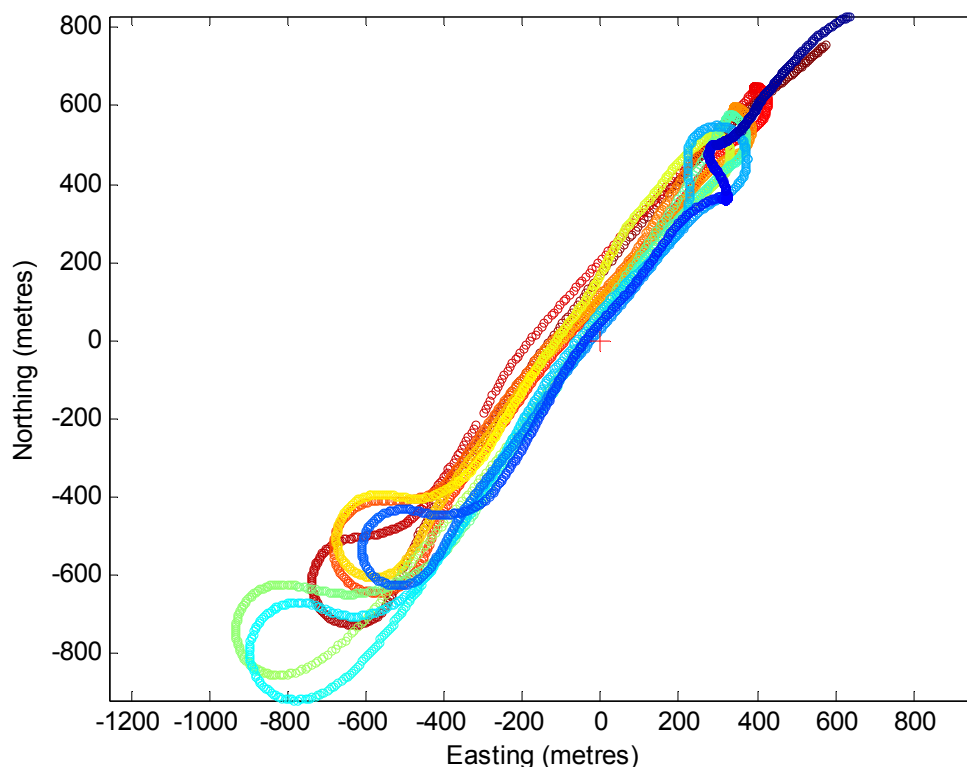
Figure 33: Example GPS trace from Quarry Point, for Star Flyte Express. GPS positions shown relative to waverecorder (red cross). Colours show times, from blue (start) to red (end).
