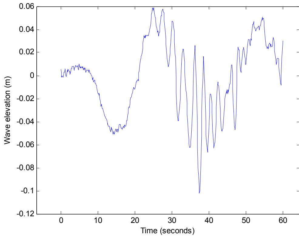
Figure 14: Measured wave elevation for River Lady on 2 nd Feb 2010, passing waverecorder at 15:27:21
