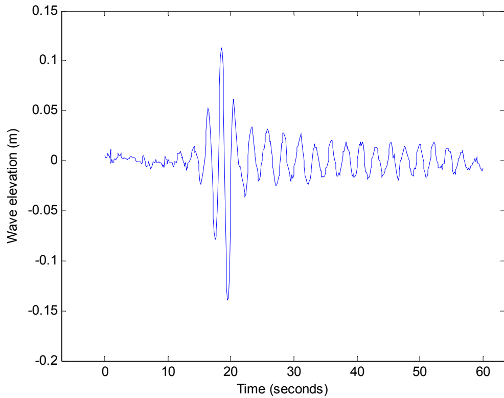
Figure 12: Measured wave elevation for Quintrex Freedom Sport 570 example case (largest wave height): 7.2 knots at 09:46
