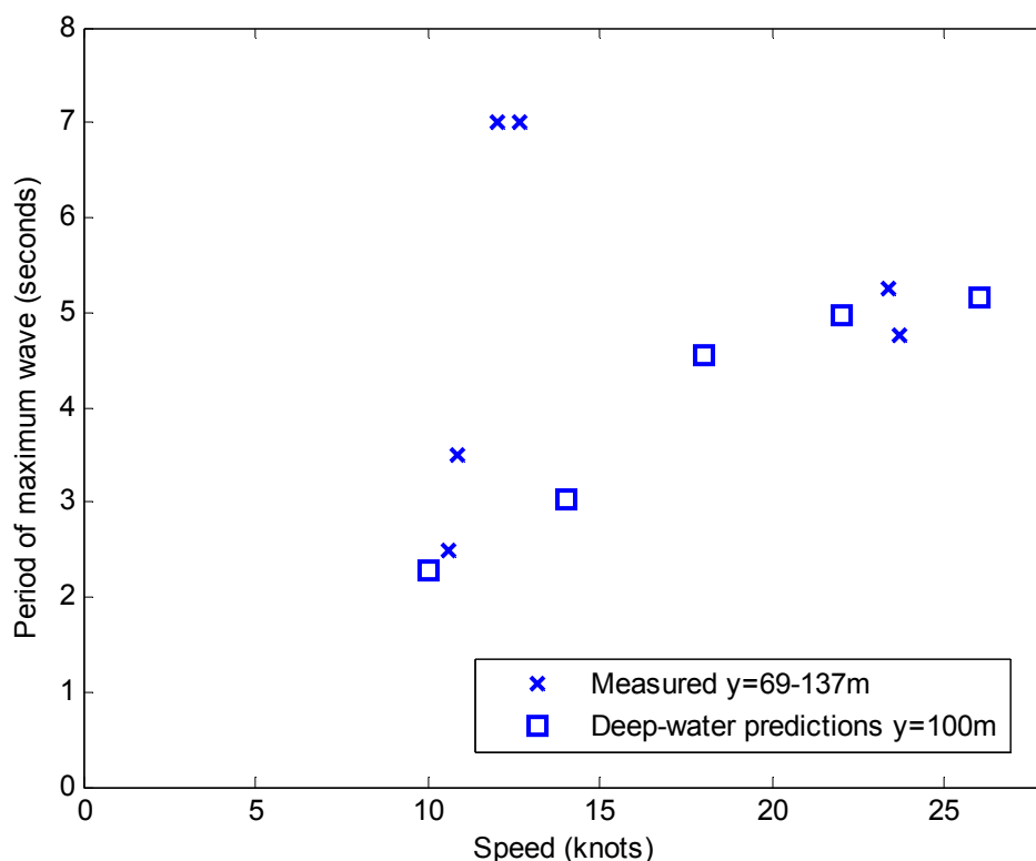
Figure 62: Comparison between measured wave periods and deep-water predictions for distant-approach trials of Star Flyte Express at Quarry Point
