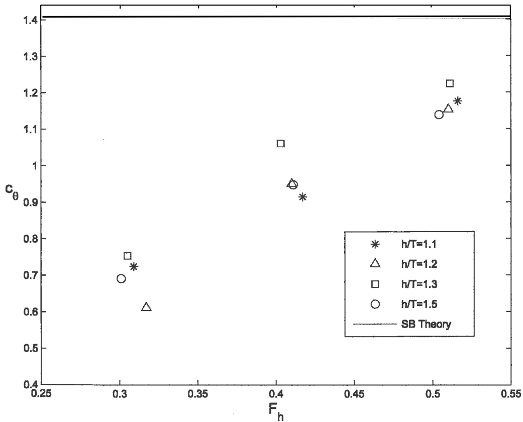
Fig. 5 Trim coefficient c_\theta as a function of depth Froude number F_h for different depth/draft ( h/T ) ratios
