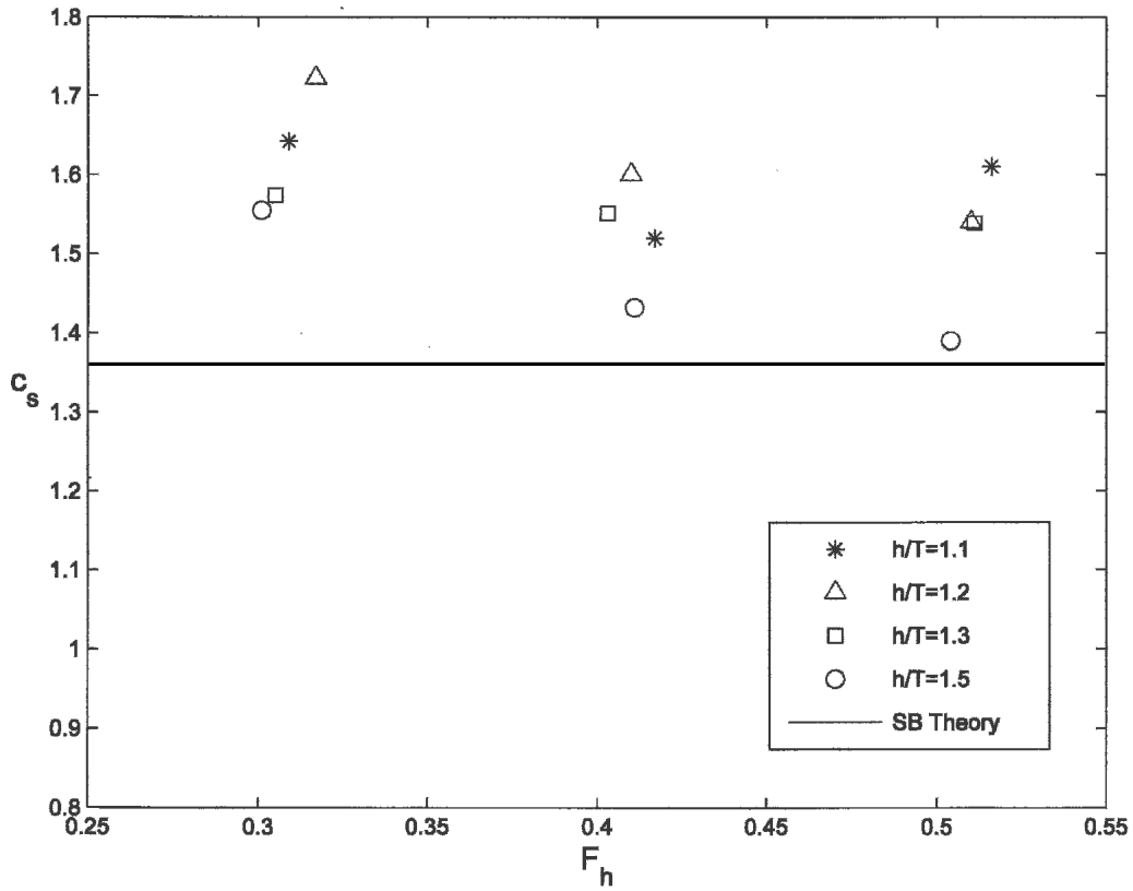
Fig. 4 LCF sinkage coefficient c_s as a function of depth Froude number F_h for different depth/draft ( h/T ) ratios
