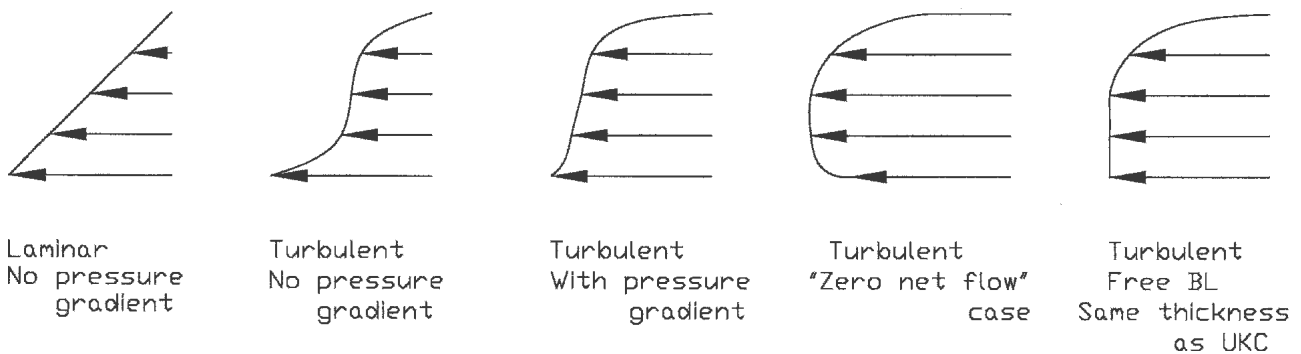
Fig. 2 Comparison of mean velocity profiles for Couette flow between two plates
