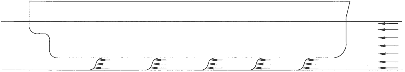
Fig. 3 Suggested model for flow beneath a ship at small underkeel clearance
