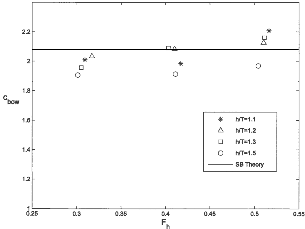
Fig. 6 Bow sinkage coefficient c_{\text{bow}} as a function of depth Froude number F_h , for different depth/draft ( h/T ) ratios
